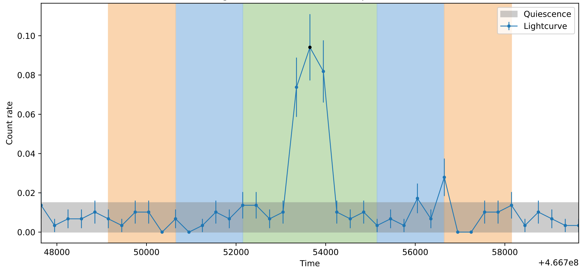
Lightcurve ObsID: 14463, Shape: None
