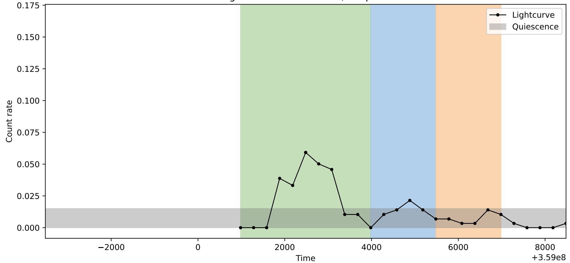
Lightcurve ObsID: 10556, Shape: 1
