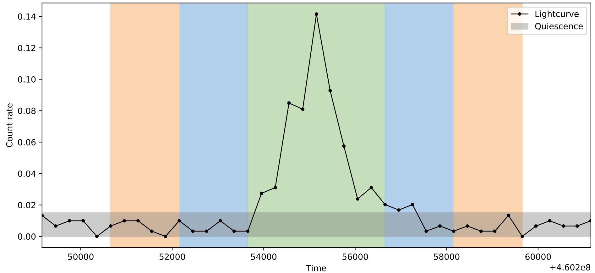
Lightcurve ObsID: 13838, Shape: 1
