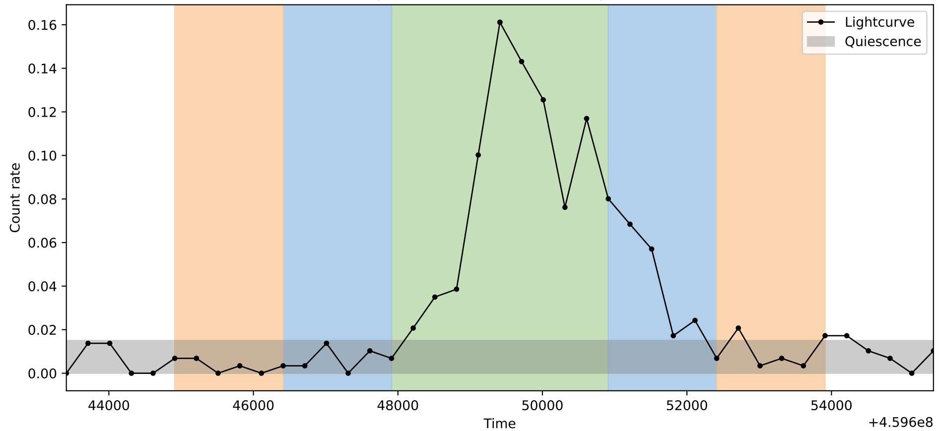
Lightcurve ObsID: 13839, Shape: 2
