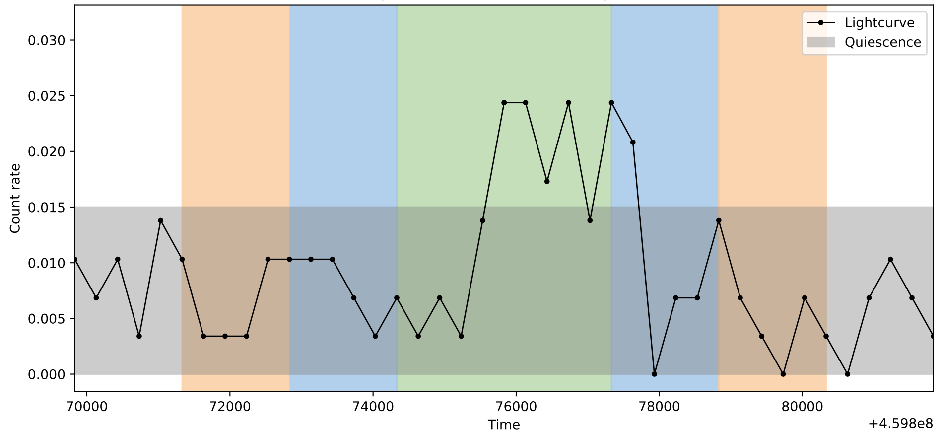
Lightcurve ObsID: 13840, Shape: 1
