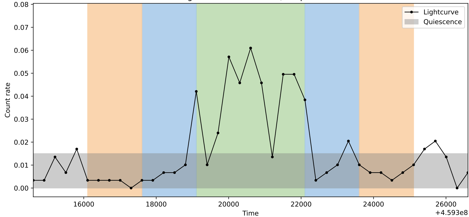
Lightcurve ObsID: 13842, Shape: 2
