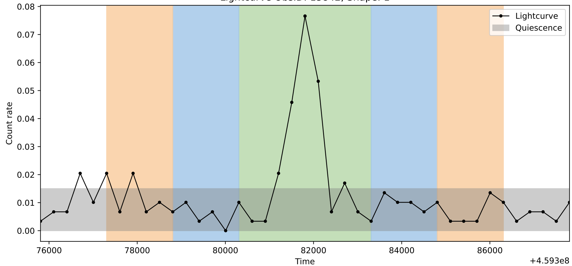
Lightcurve ObsID: 13842, Shape: 1
