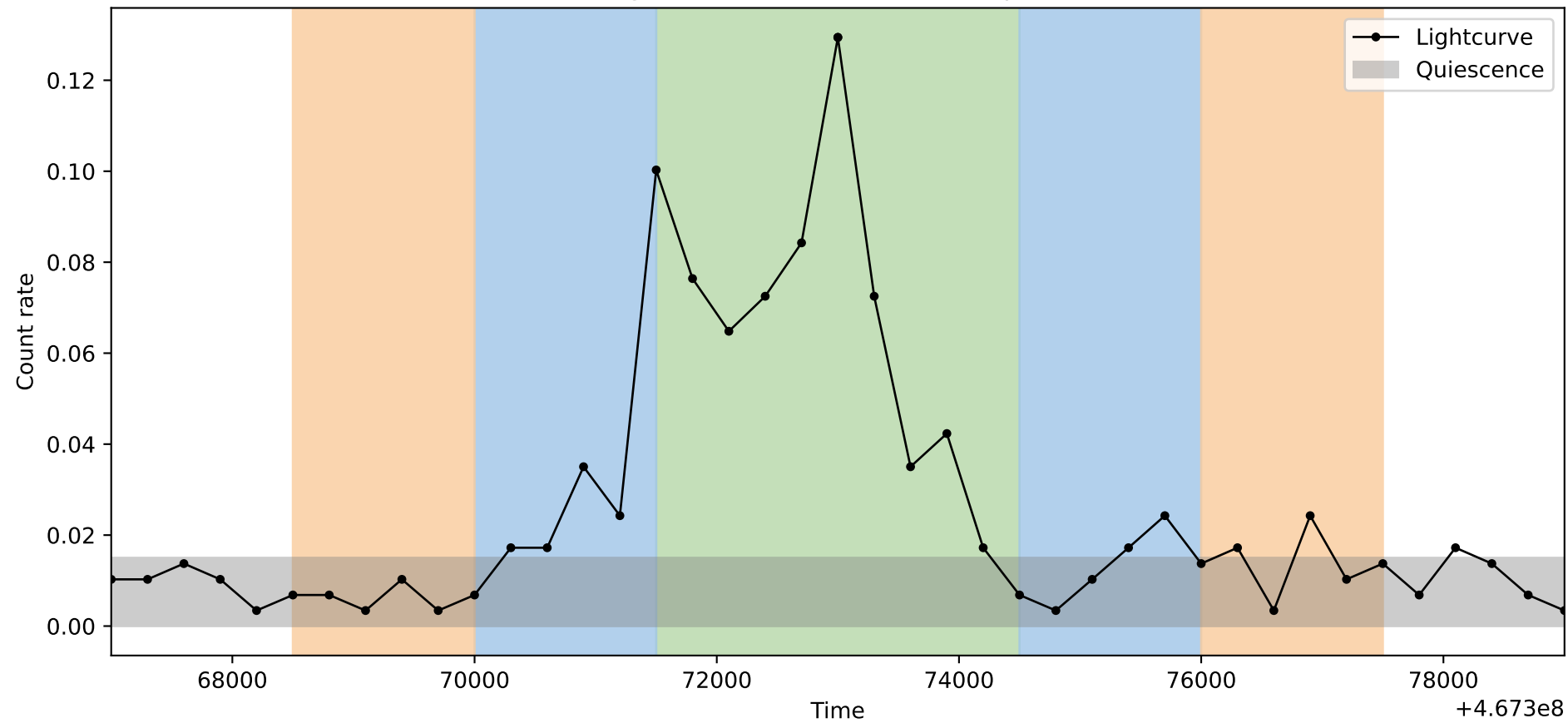
Lightcurve ObsID: 13843, Shape: 3
