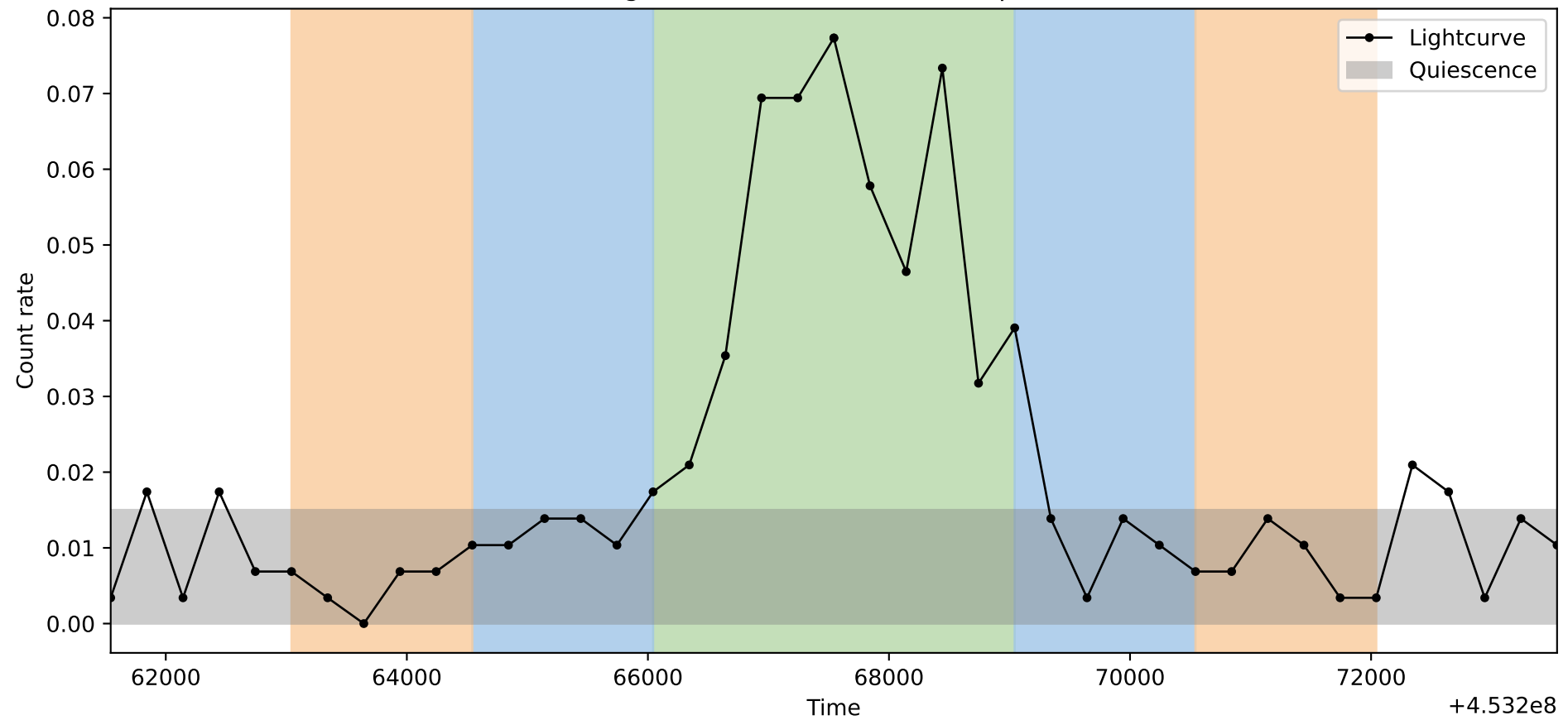
Lightcurve ObsID: 13849, Shape: 1
