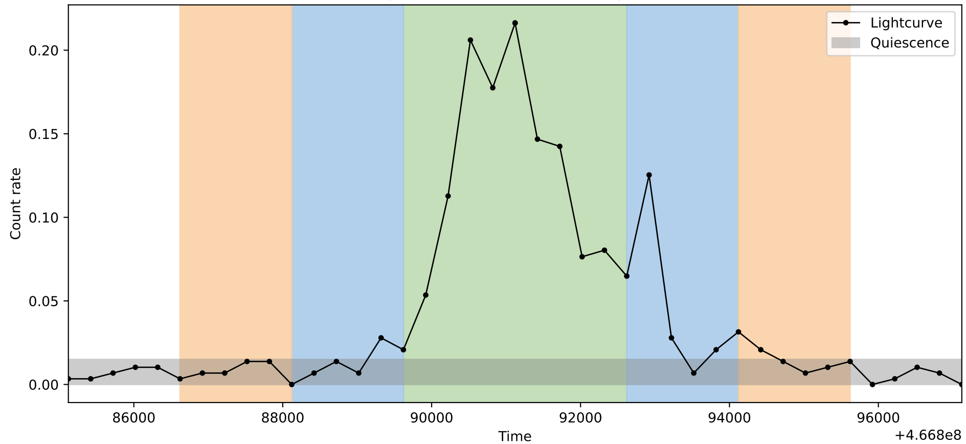
Lightcurve ObsID: 13851, Shape: 2
