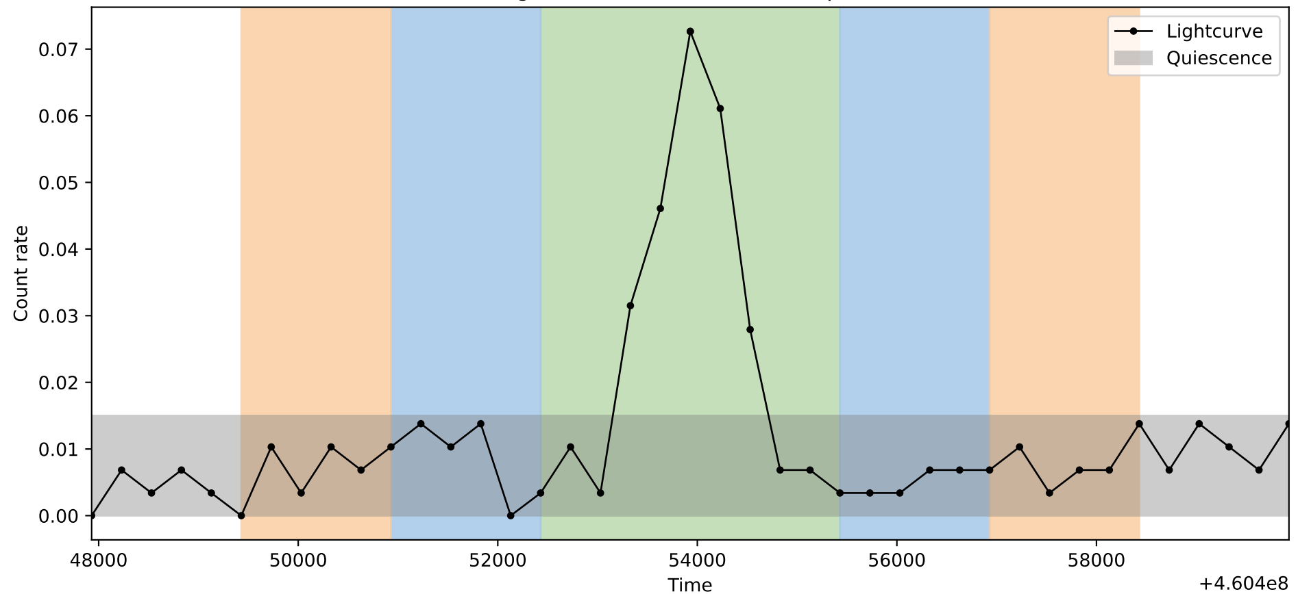
Lightcurve ObsID: 13852, Shape: 1
