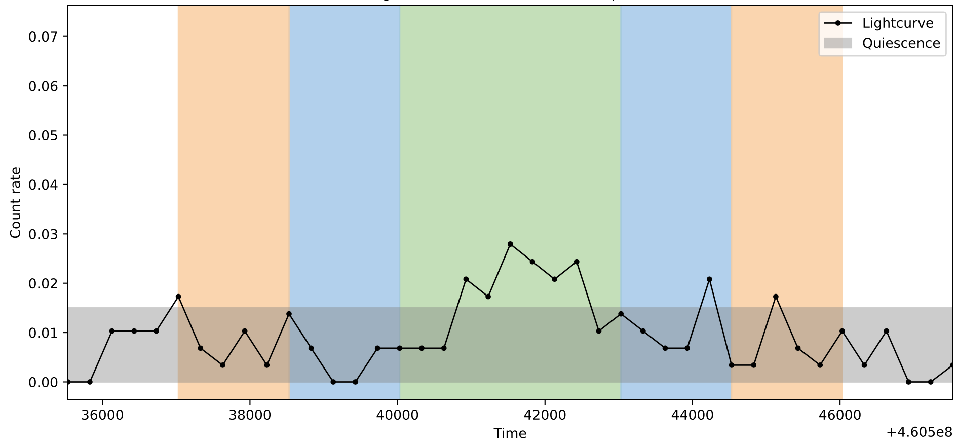
Lightcurve ObsID: 13852, Shape: 1
