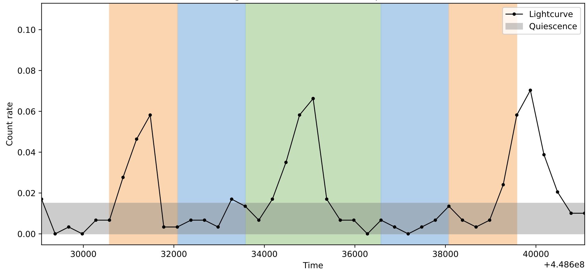
Lightcurve ObsID: 13854, Shape: 1
