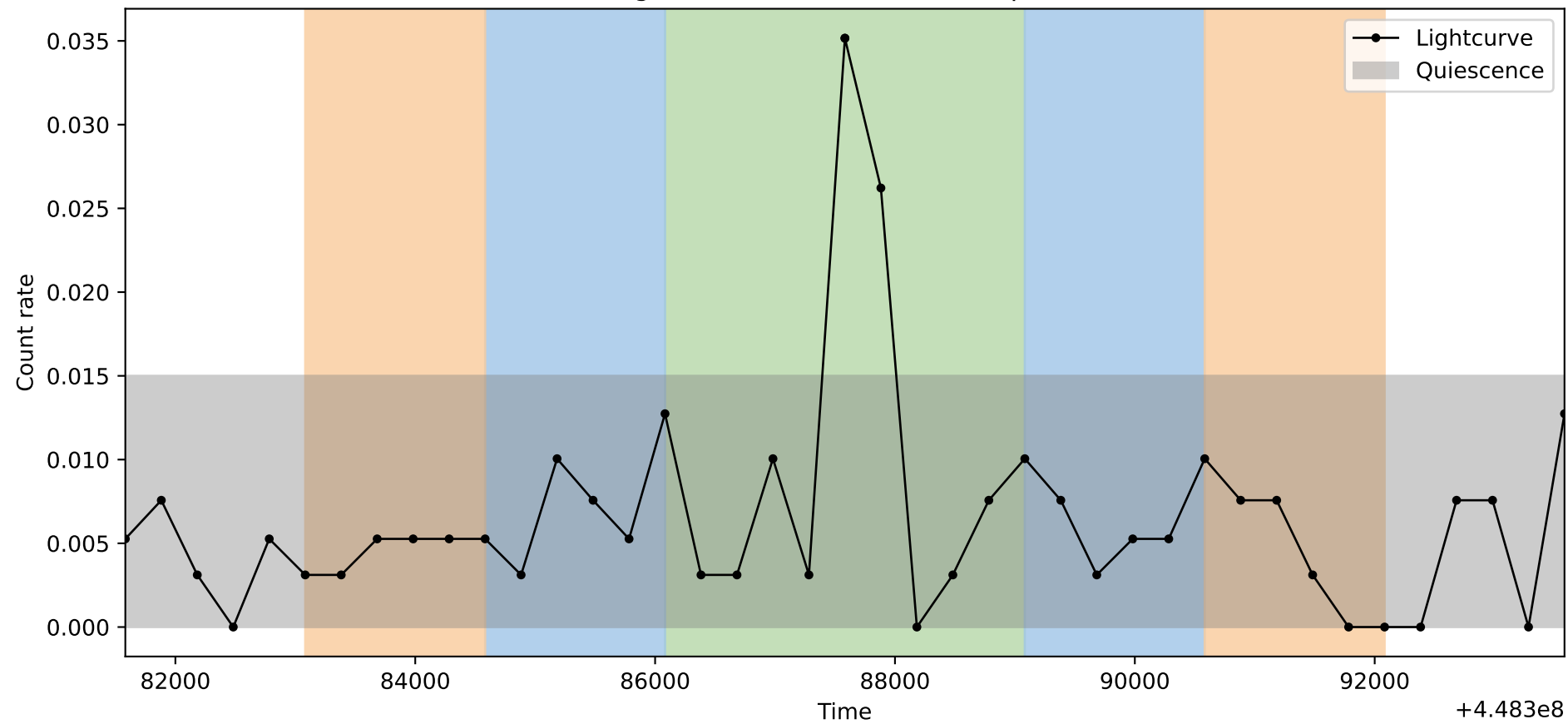
Lightcurve ObsID: 13857, Shape: 1
