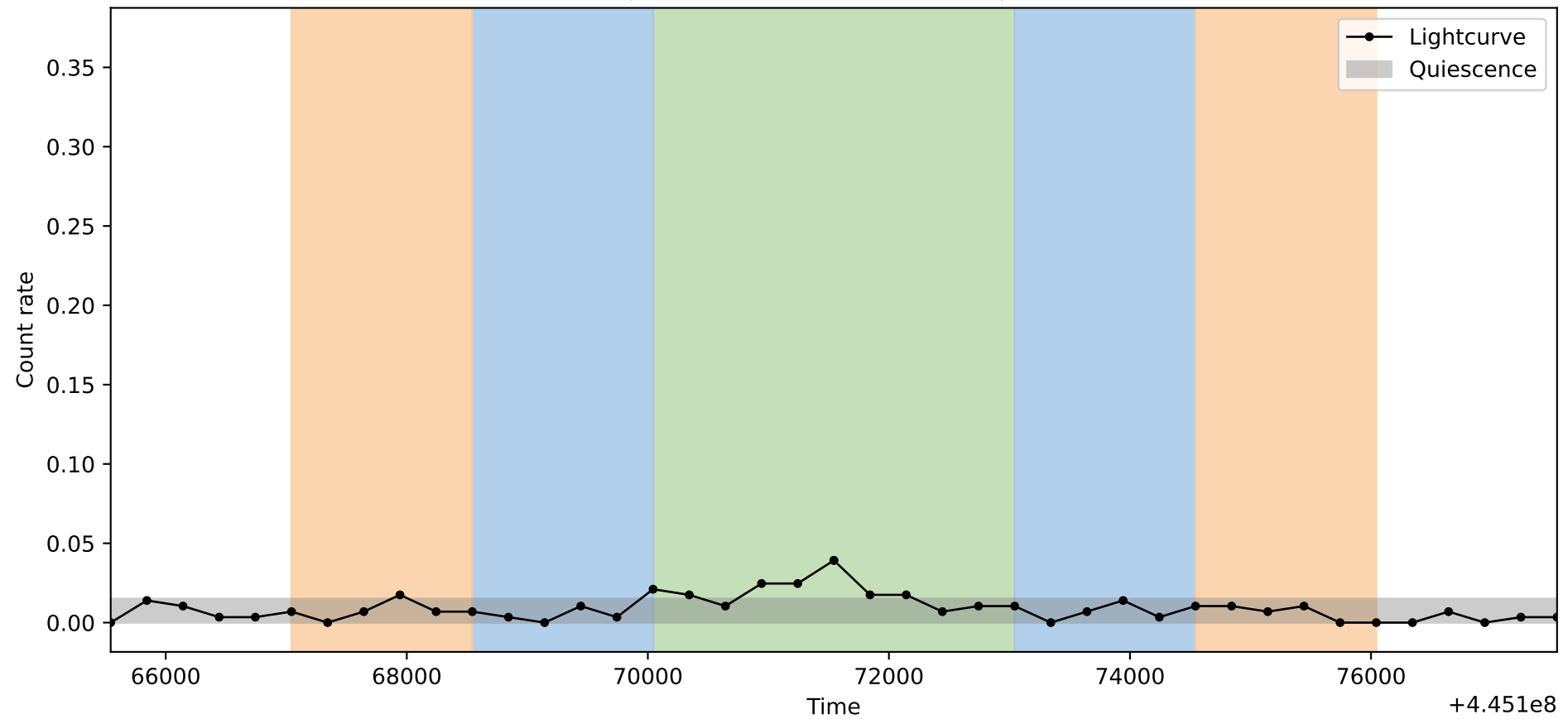
Lightcurve ObsID: 14392, Shape: 1
