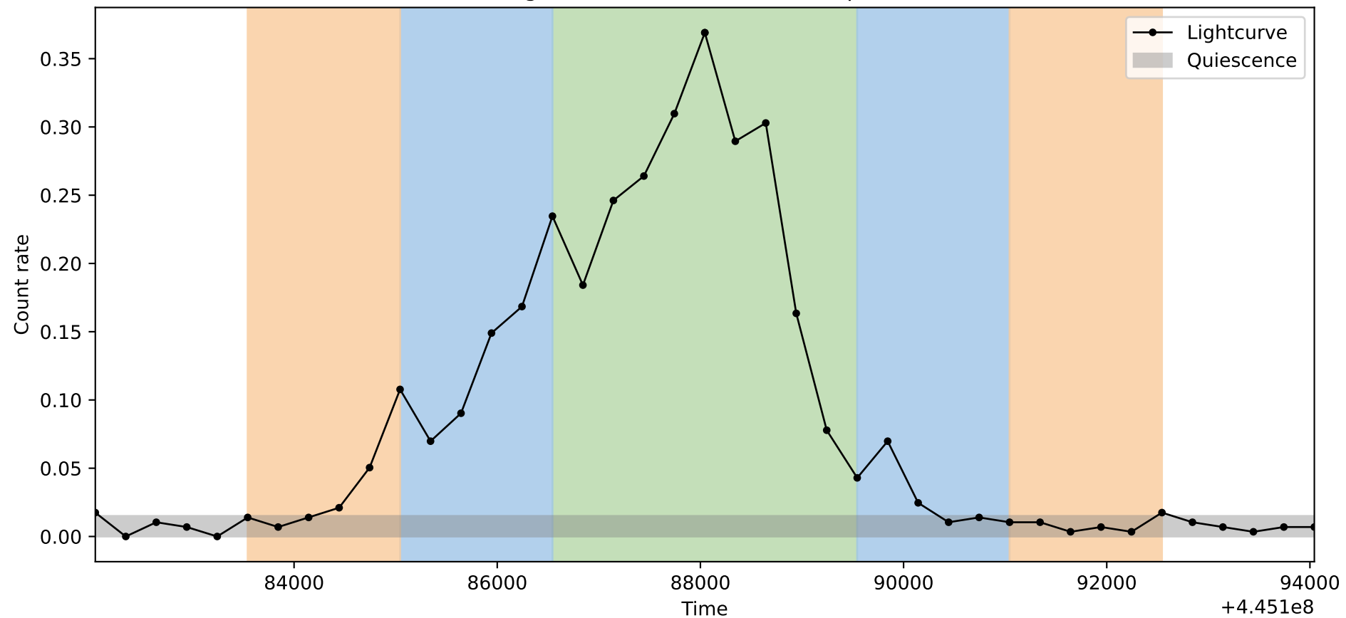
Lightcurve ObsID: 14392, Shape: 3
