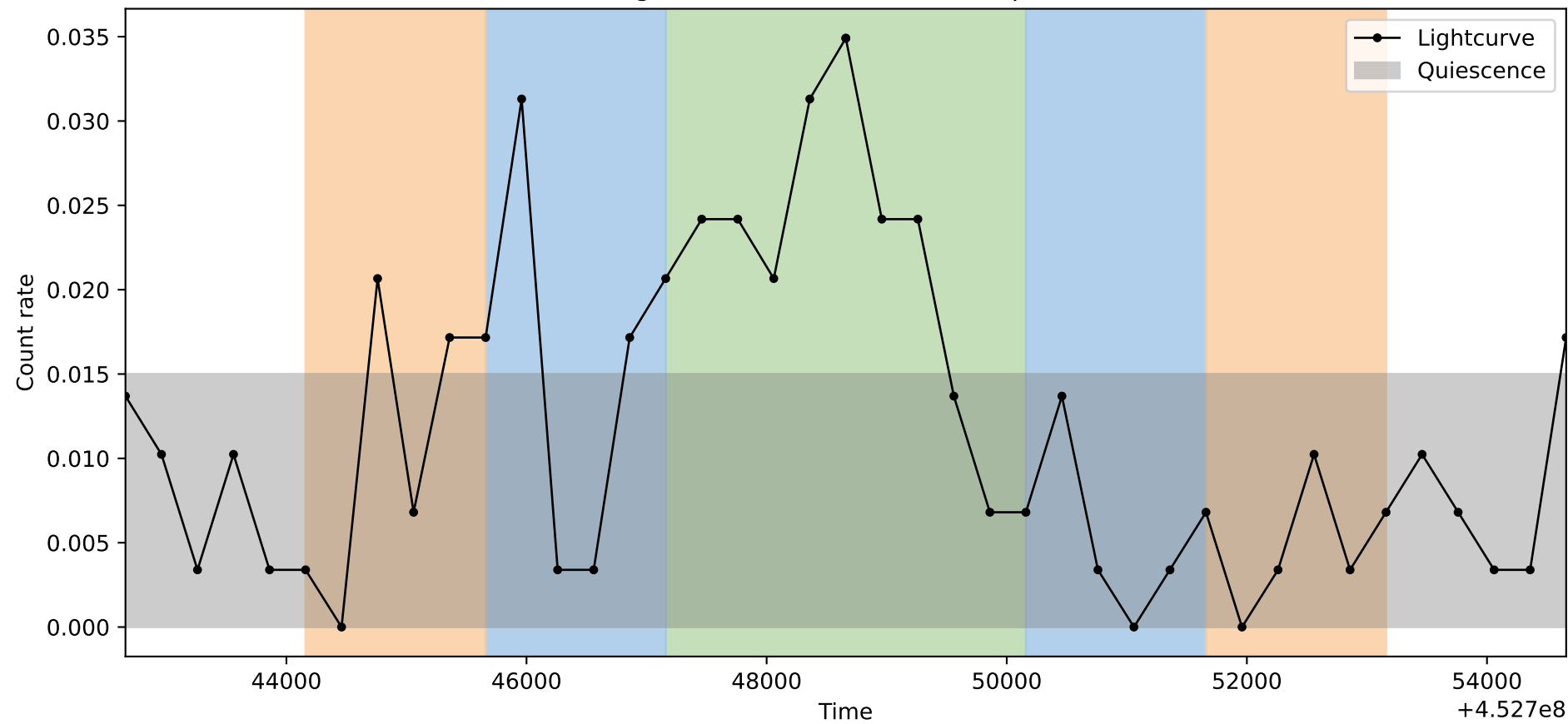
Lightcurve ObsID: 14427, Shape: 2
