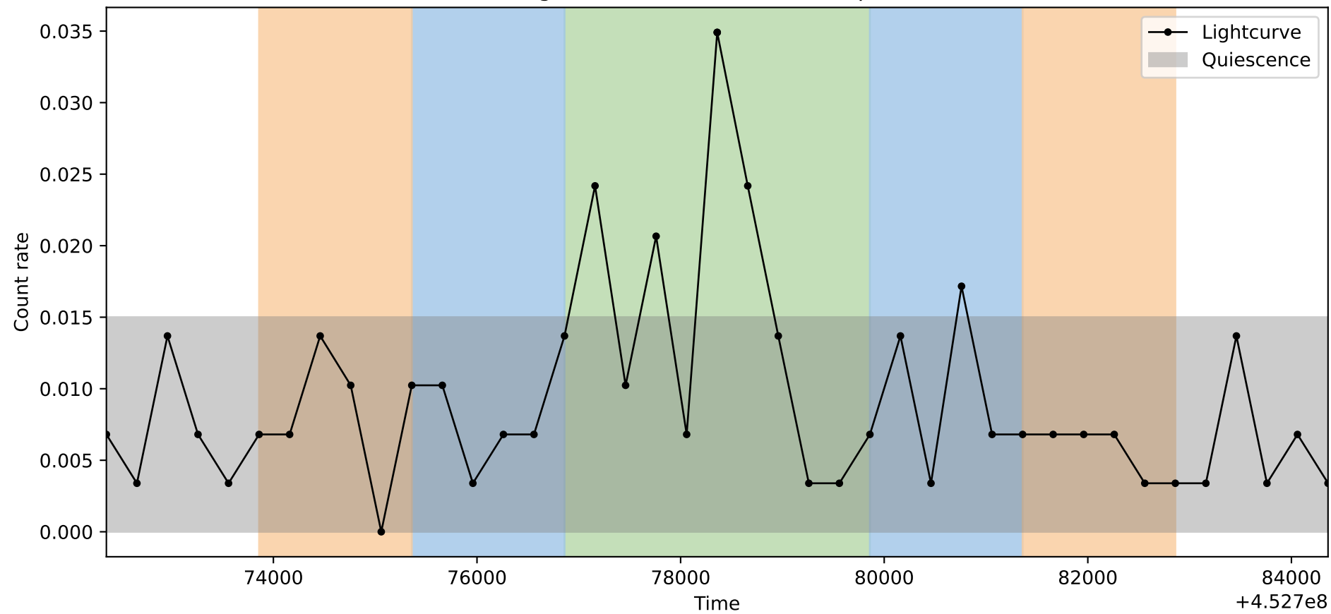
Lightcurve ObsID: 14427, Shape: 1
