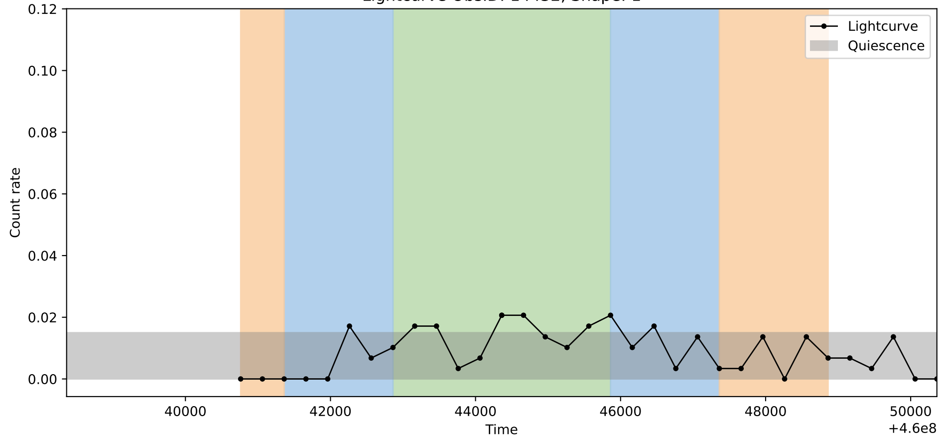
Lightcurve ObsID: 14432, Shape: 1
