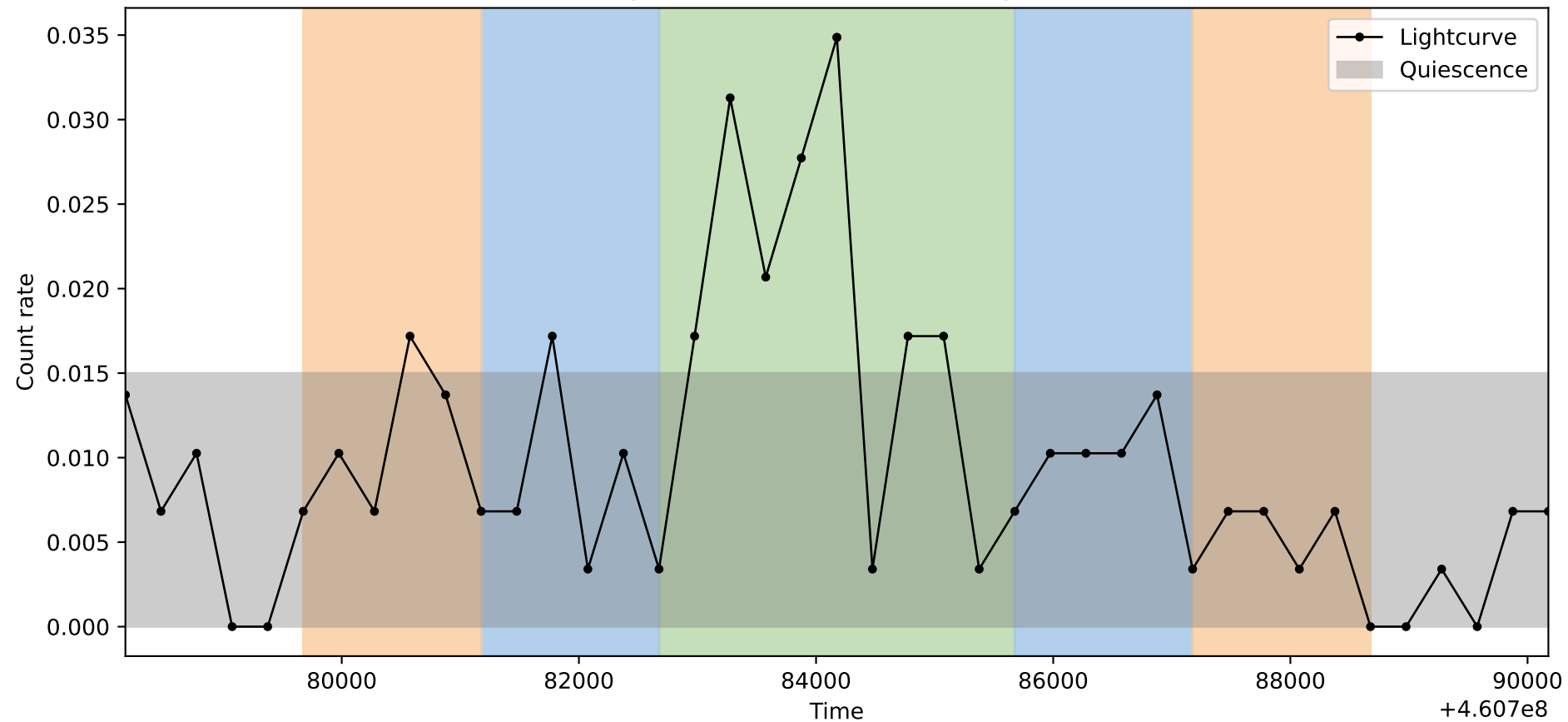
Lightcurve ObsID: 14439, Shape: 1
