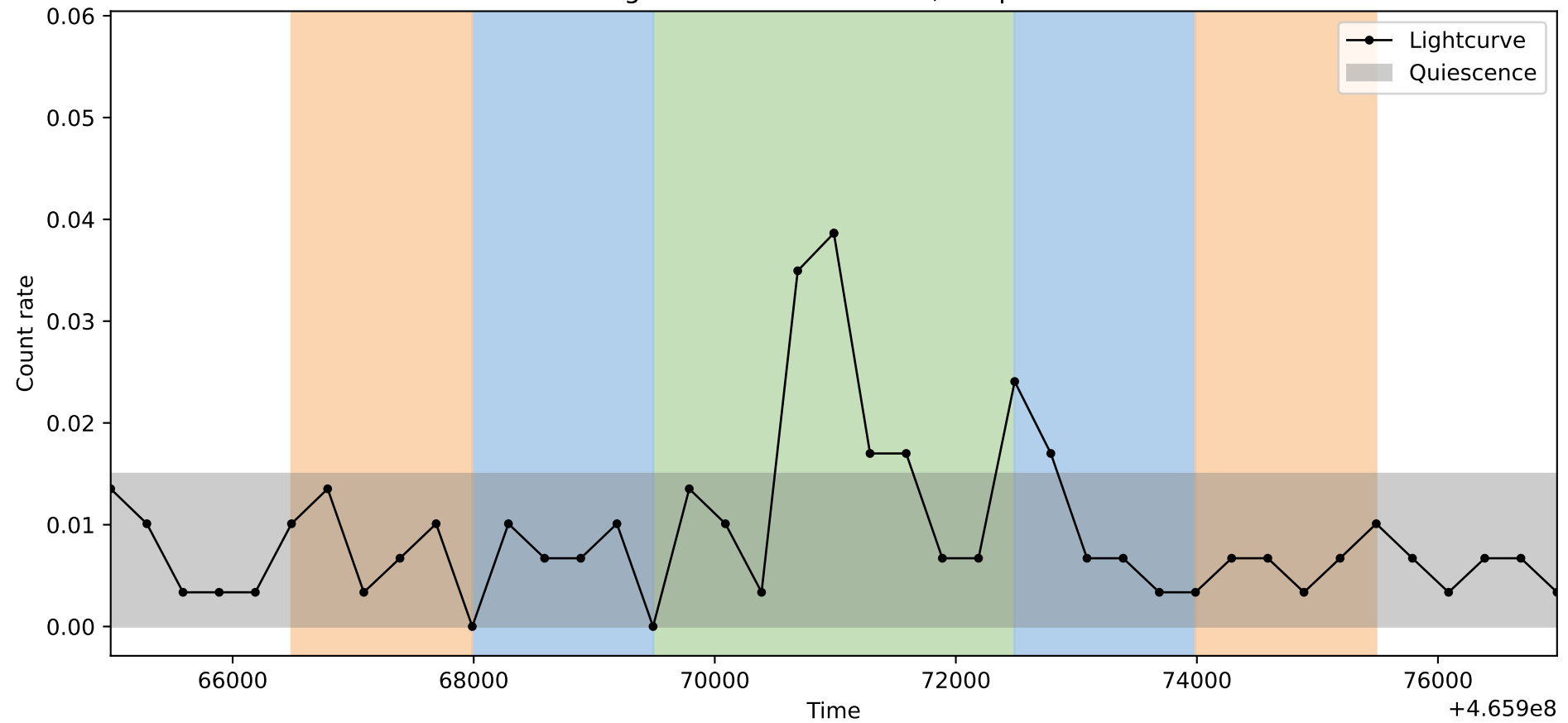
Lightcurve ObsID: 14462, Shape: 1
