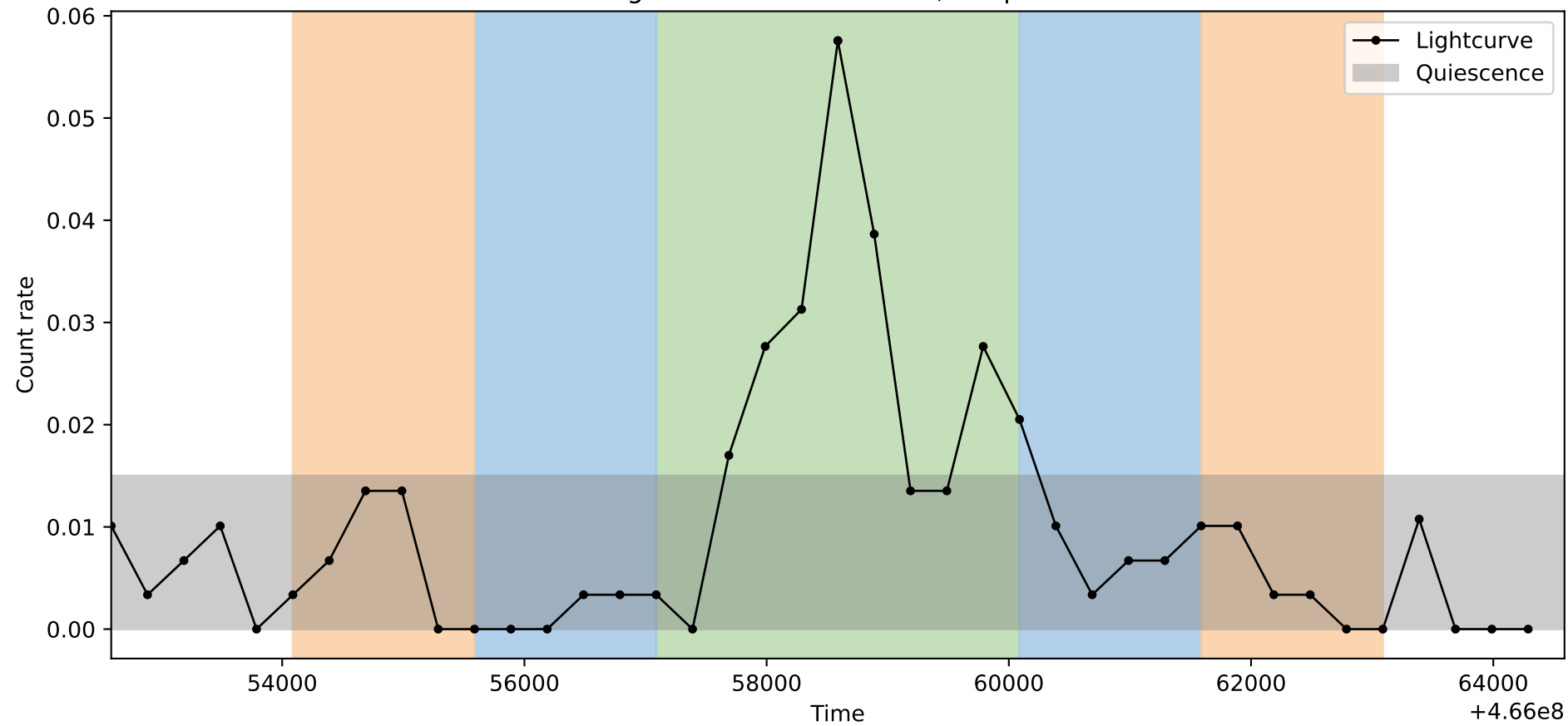
Lightcurve ObsID: 14462, Shape: 2
