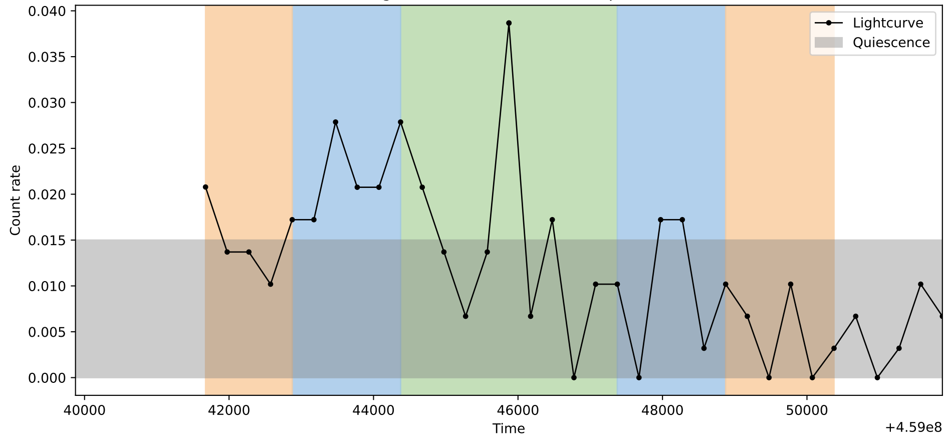
Lightcurve ObsID: 14465, Shape: 2
