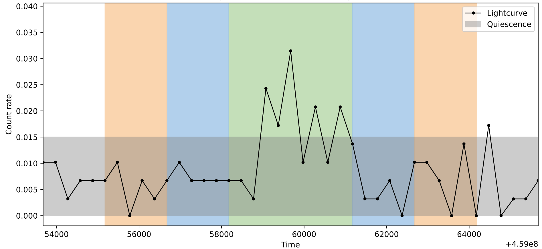
Lightcurve ObsID: 14465, Shape: 1
