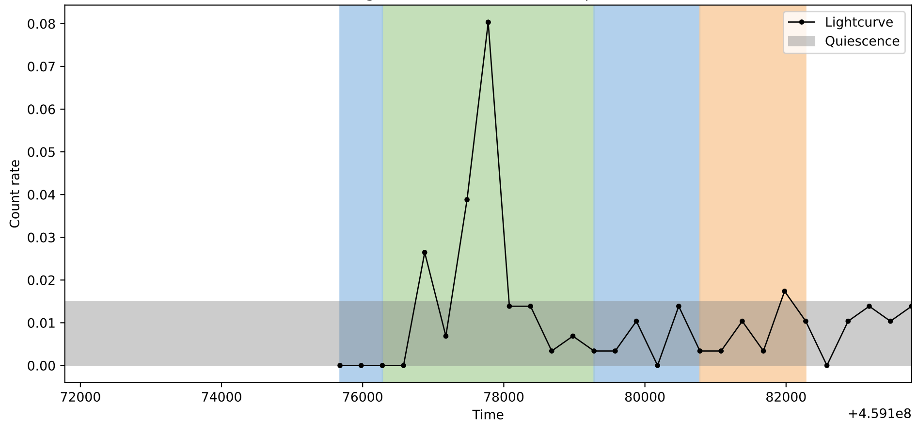
Lightcurve ObsID: 14466, Shape: 1
