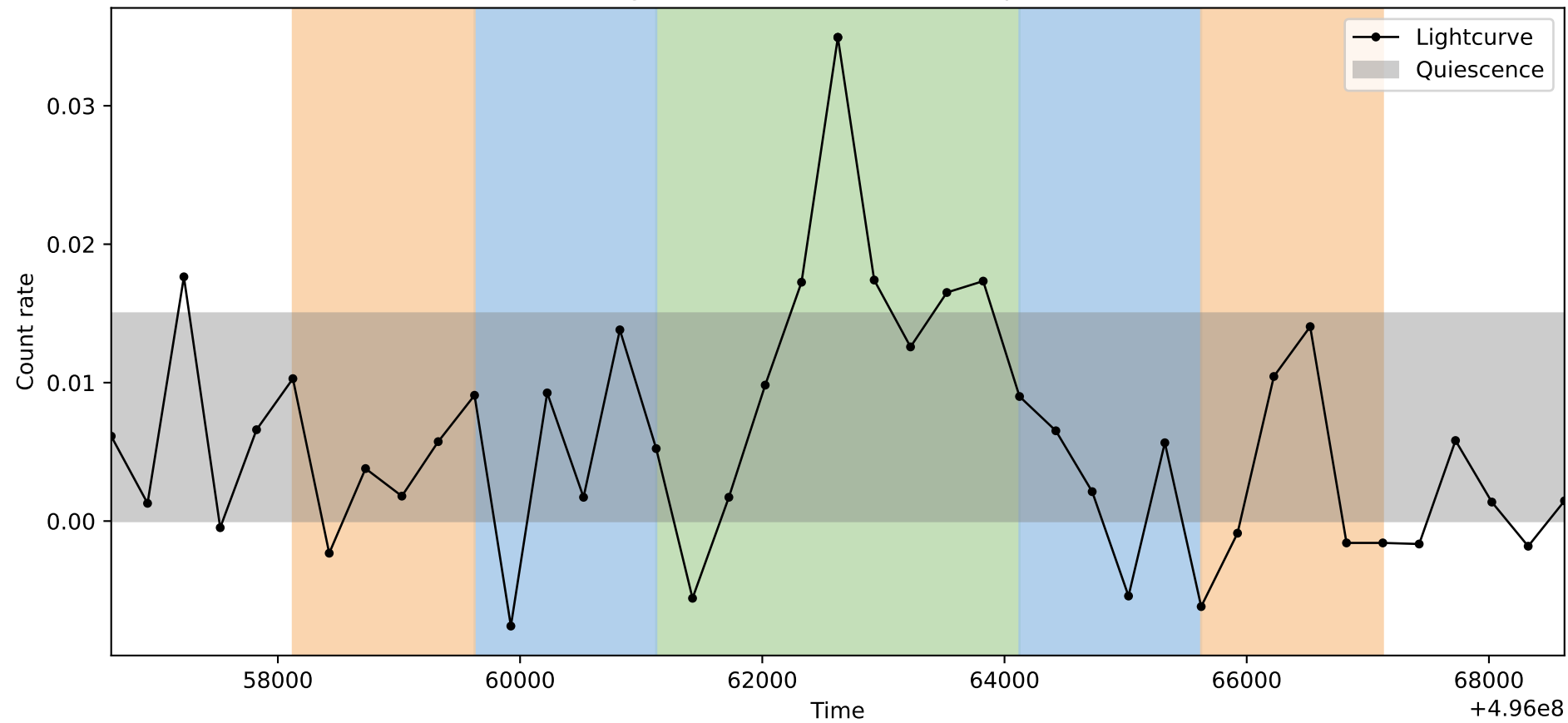
Lightcurve ObsID: 14944, Shape: 2
