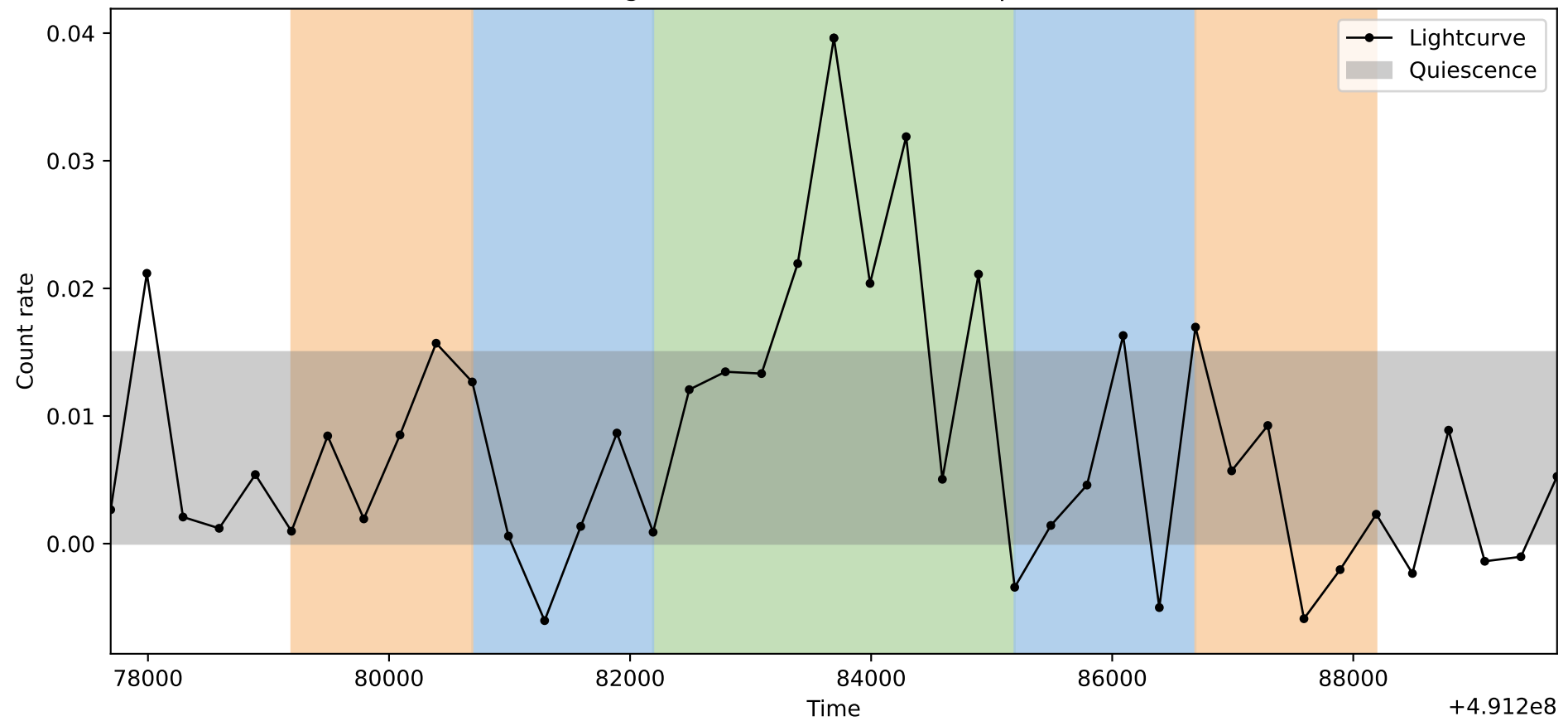
Lightcurve ObsID: 15041, Shape: 1
