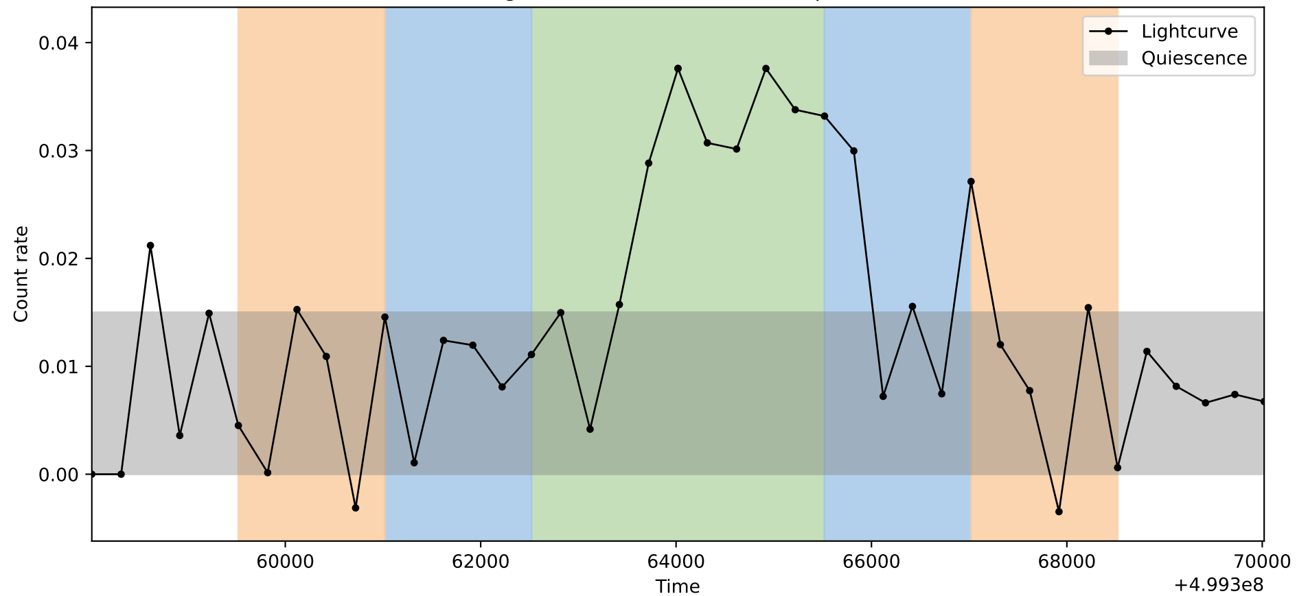
Lightcurve ObsID: 15045, Shape: 2
