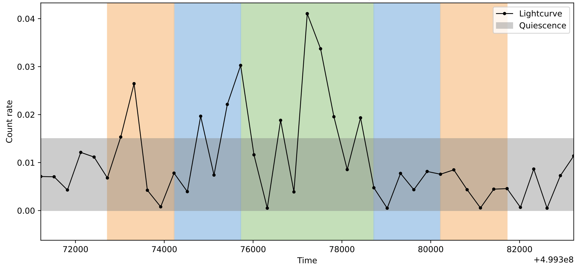
Lightcurve ObsID: 15045, Shape: 1
