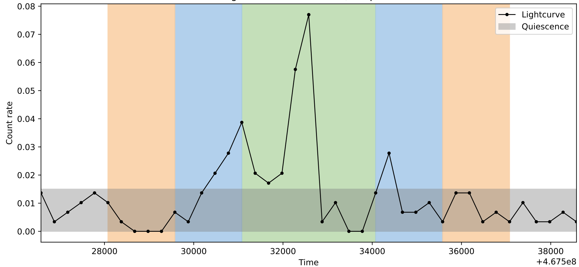
Lightcurve ObsID: 15570, Shape: 2
