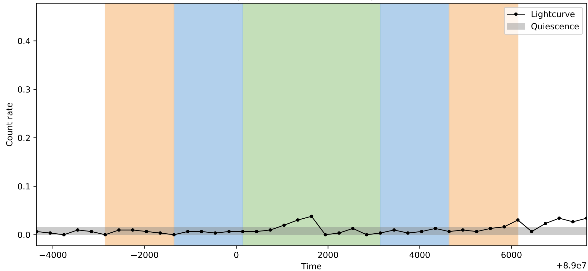
Lightcurve ObsID: 1561, Shape: 1
