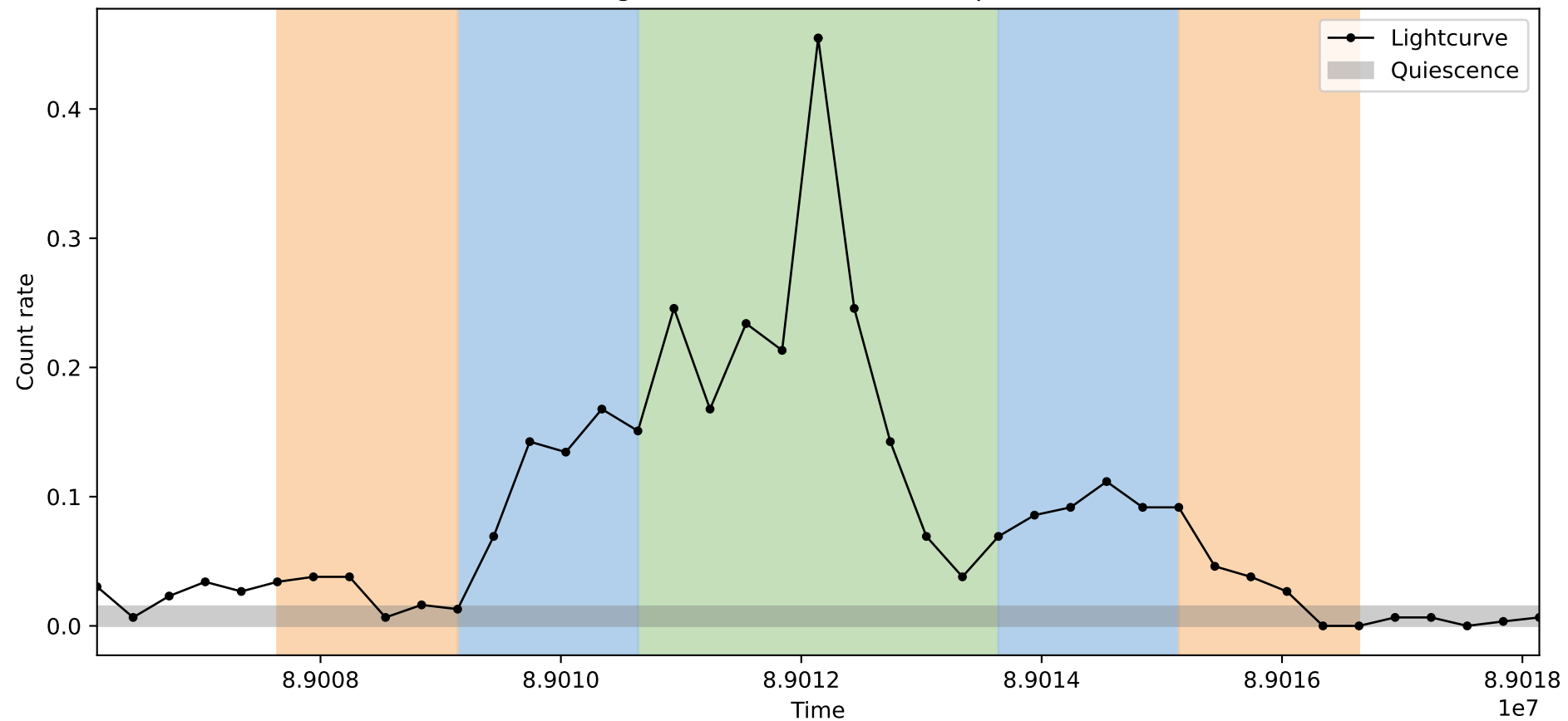
Lightcurve ObsID: 1561, Shape: 3
