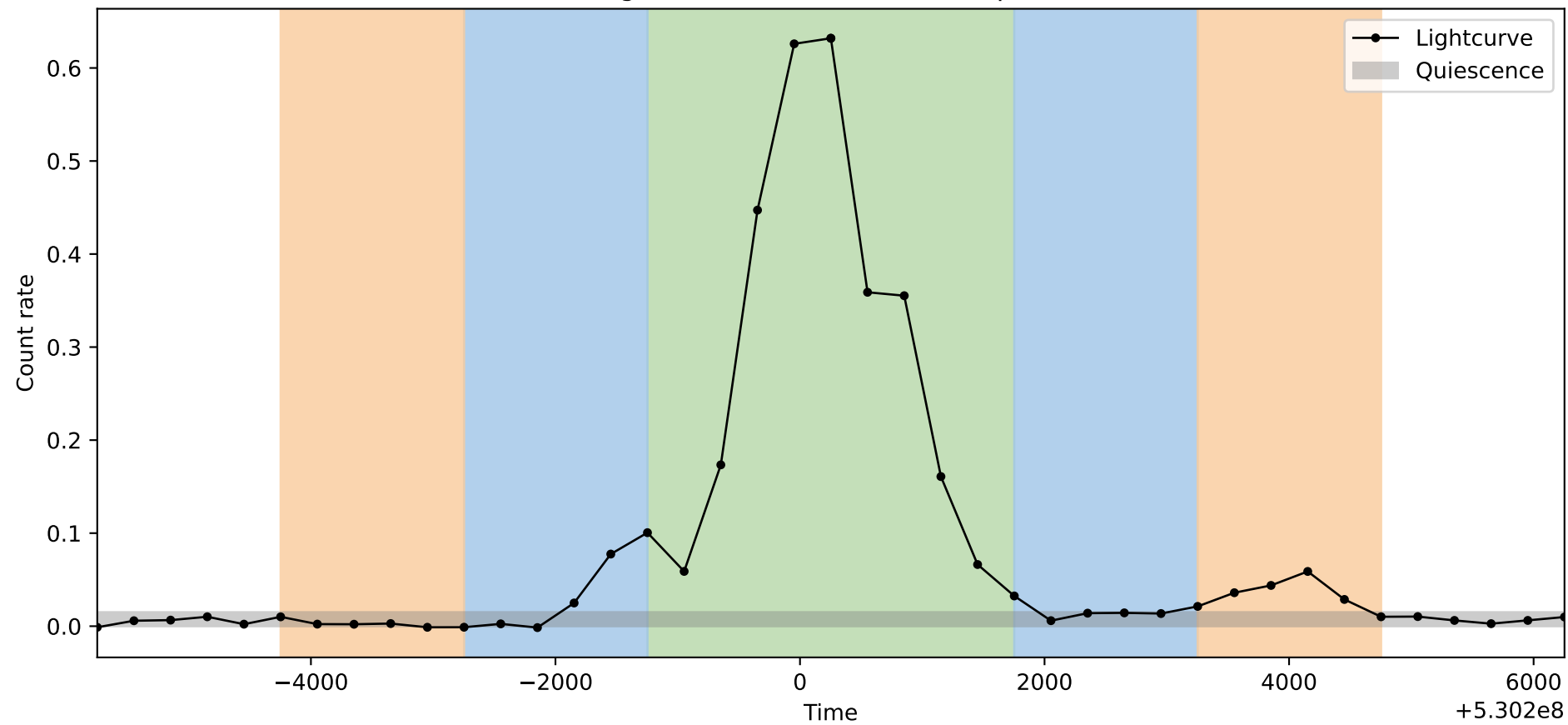
Lightcurve ObsID: 16218, Shape: 3
