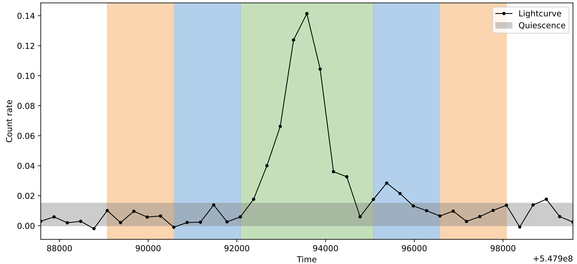
Lightcurve ObsID: 16966, Shape: 2
