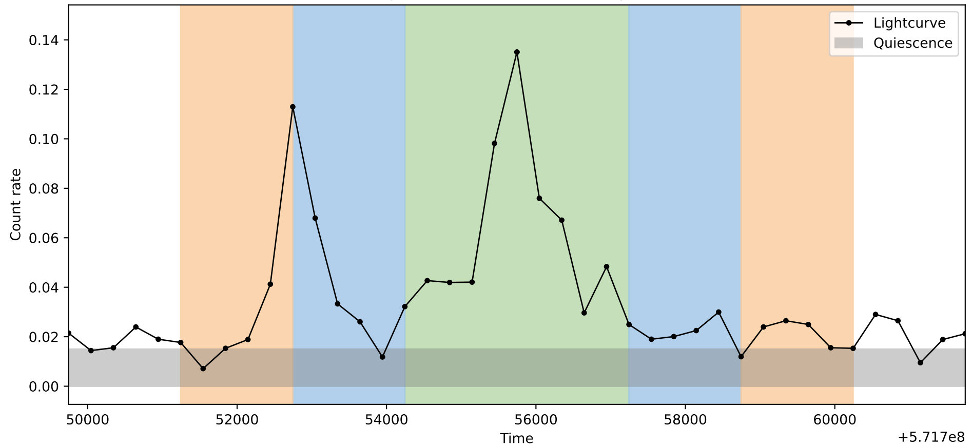
Lightcurve ObsID: 18055, Shape: 3
