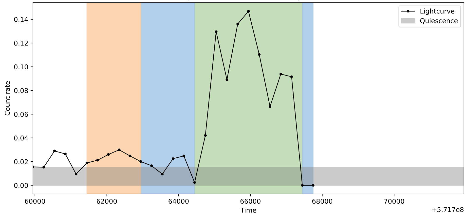
Lightcurve ObsID: 18055, Shape: 2
