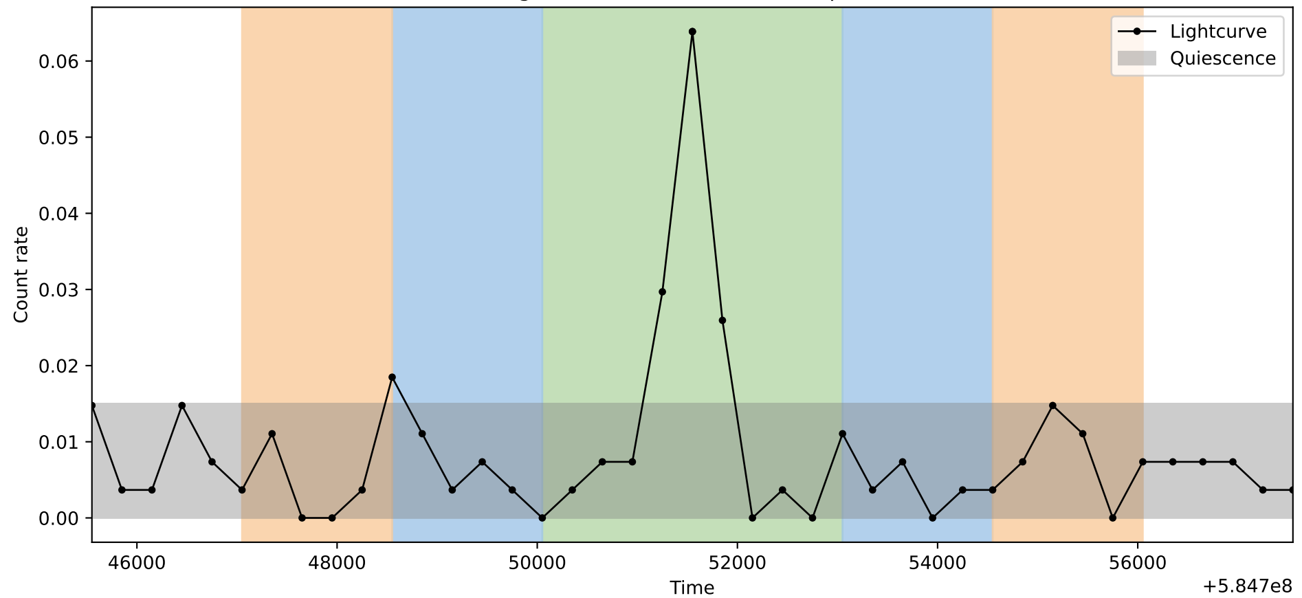
Lightcurve ObsID: 18731, Shape: 1
