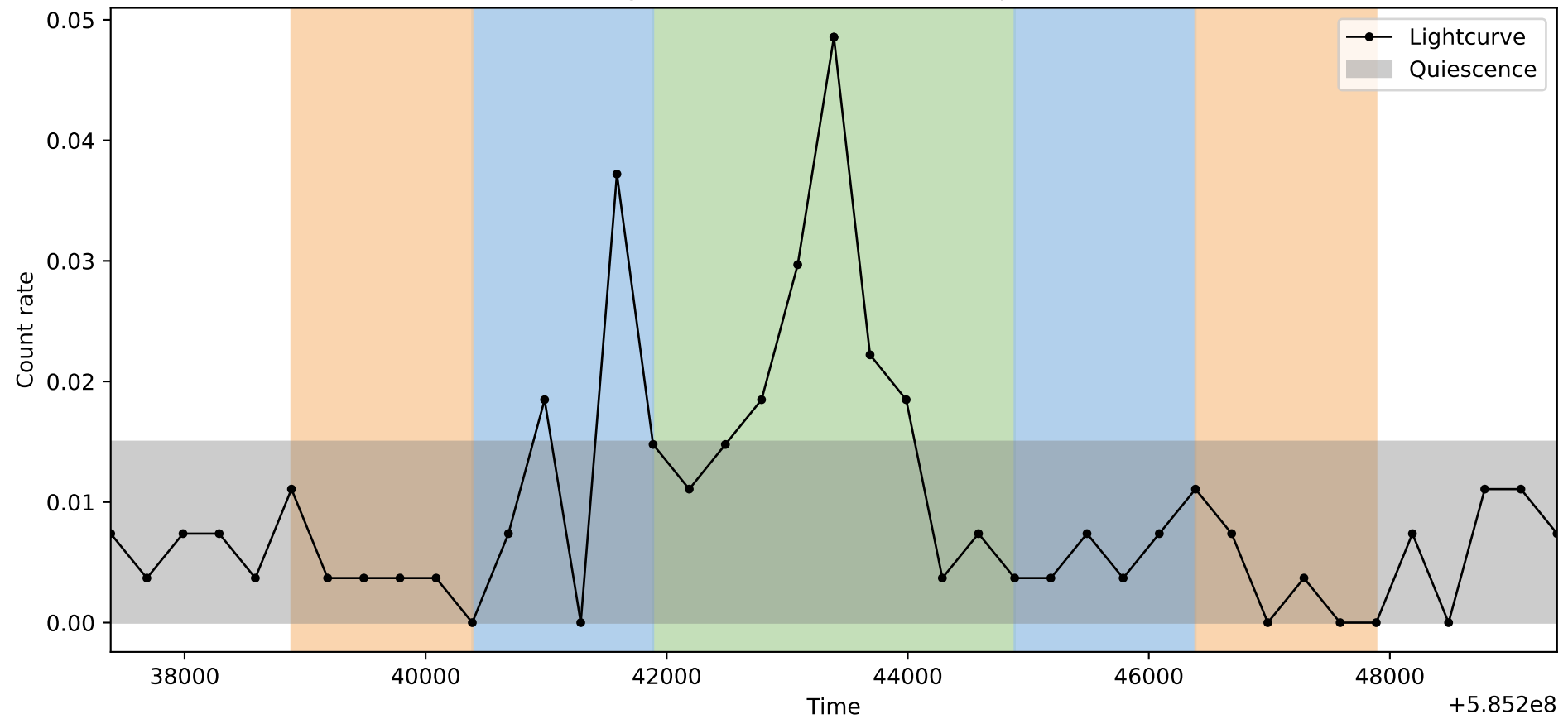
Lightcurve ObsID: 18732, Shape: 2
