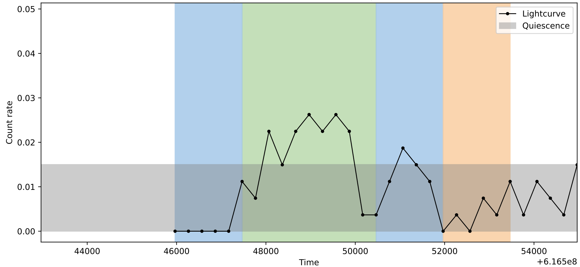
Lightcurve ObsID: 19703, Shape: 1
