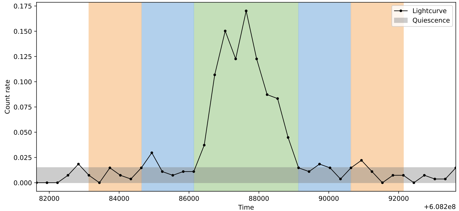
Lightcurve ObsID: 20041, Shape: 1
