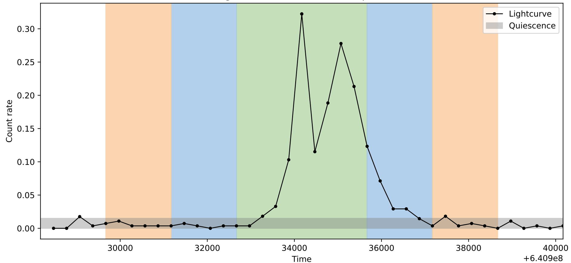
Lightcurve ObsID: 20346, Shape: 2
