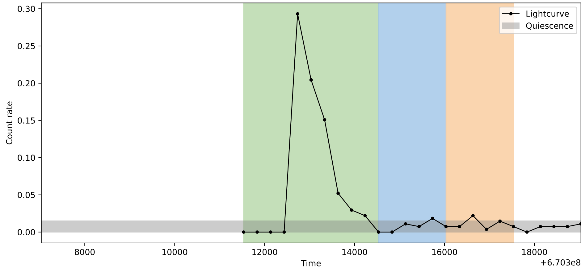
Lightcurve ObsID: 21454, Shape: 1
