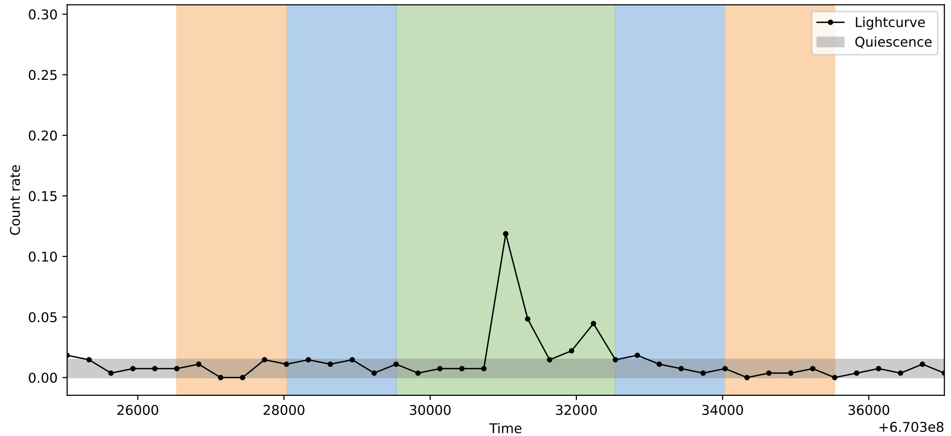
Lightcurve ObsID: 21454, Shape: 2
