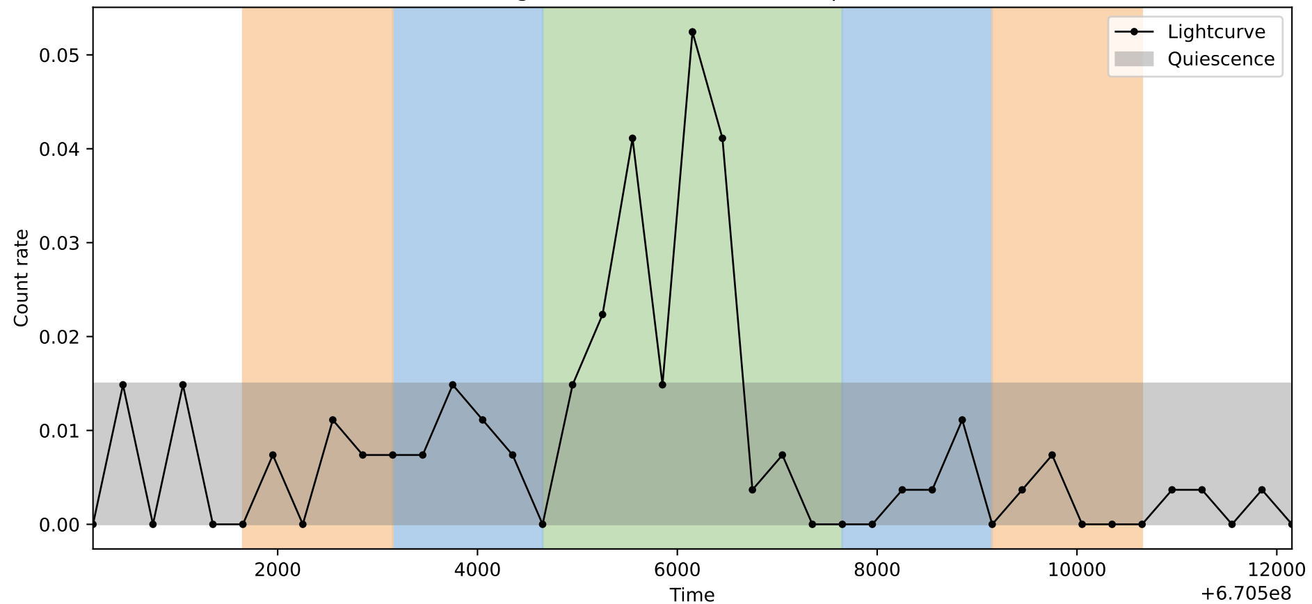
Lightcurve ObsID: 21456, Shape: 2
