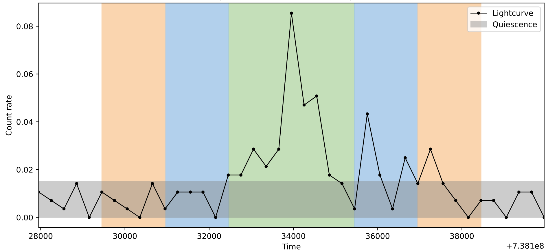
Lightcurve ObsID: 22592, Shape: 2
