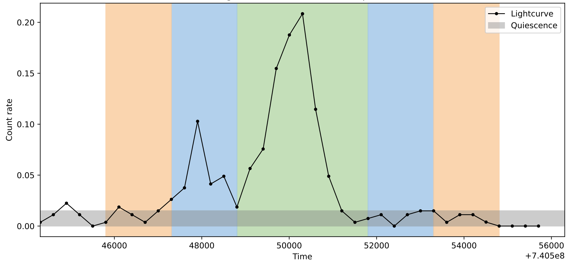
Lightcurve ObsID: 22594, Shape: 2
