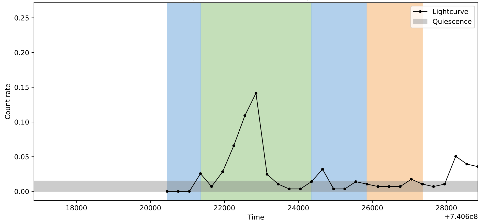
Lightcurve ObsID: 22595, Shape: 1
