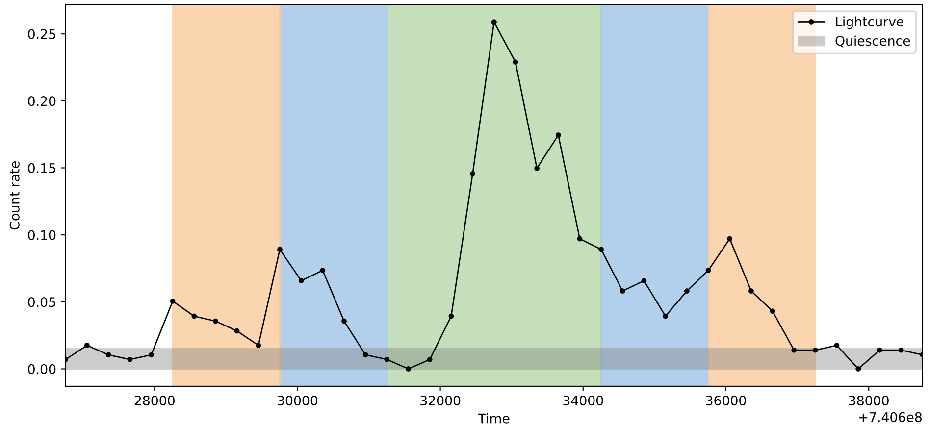
Lightcurve ObsID: 22595, Shape: 3
