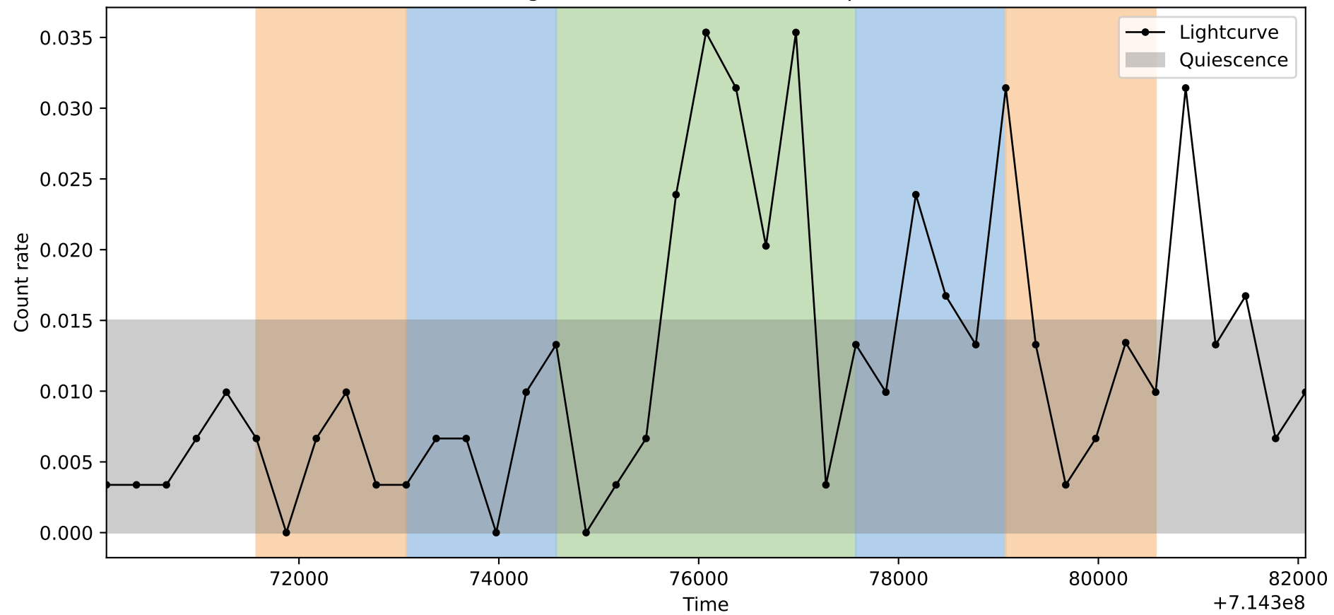
Lightcurve ObsID: 22937, Shape: 2
