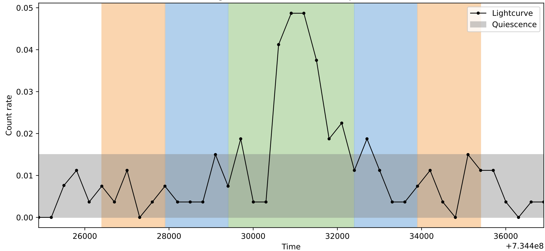
Lightcurve ObsID: 23665, Shape: 1
